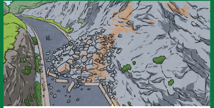
Landslide
