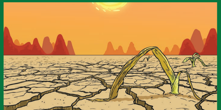
Drought
