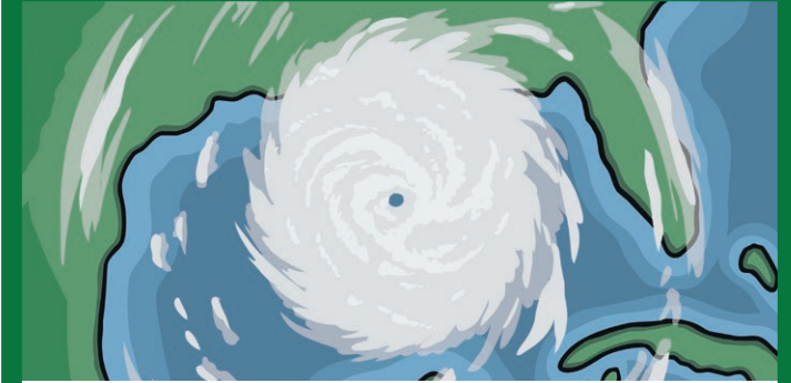
Hurricane
