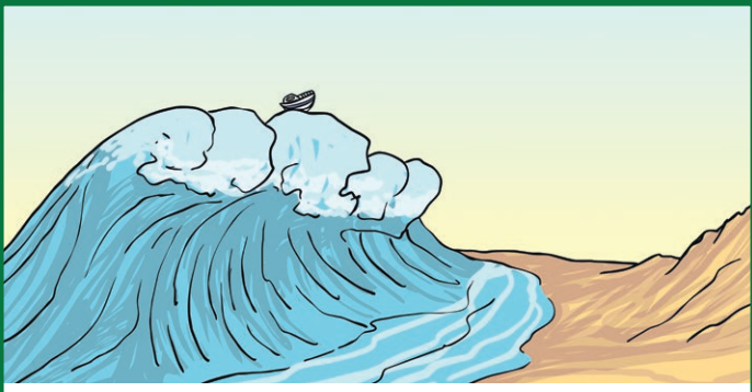
Tsunami
